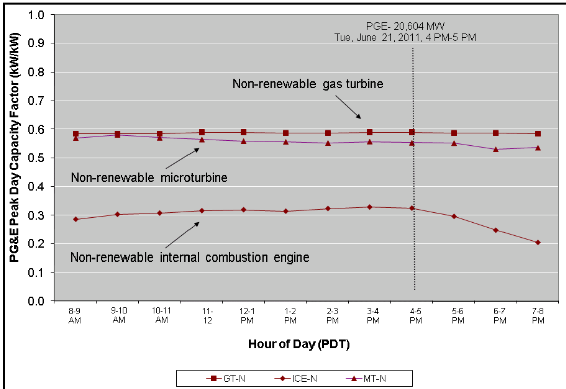
Figure A-34: 2011 IOU Peak Day Capacity Factors by Technology—PG&E
