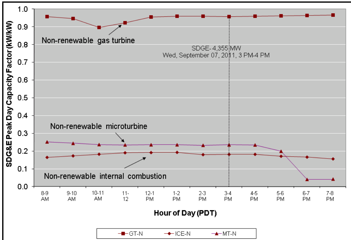
Figure A-36: 2011 IOU Peak Day Capacity Factors by Technology—SDG&E
