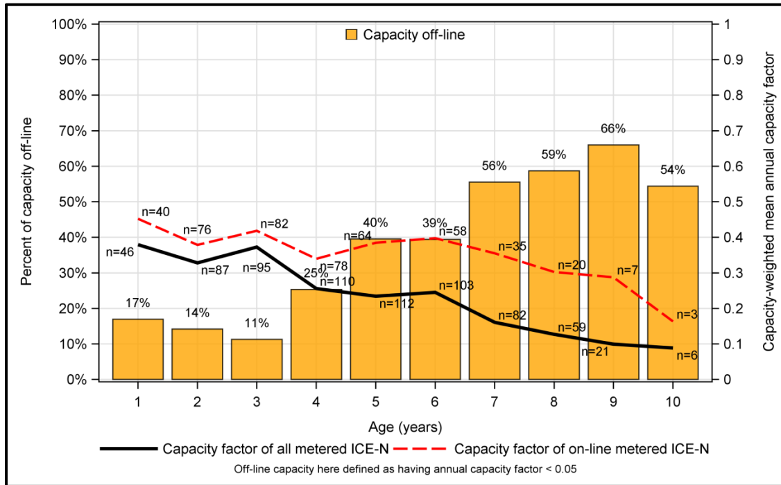
Figure A-47: ICE-N Annual Capacity Factor and Off-line by Age
