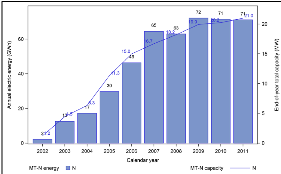
Figure A-42: MT-N Capacity and Annual Impacts by Year
