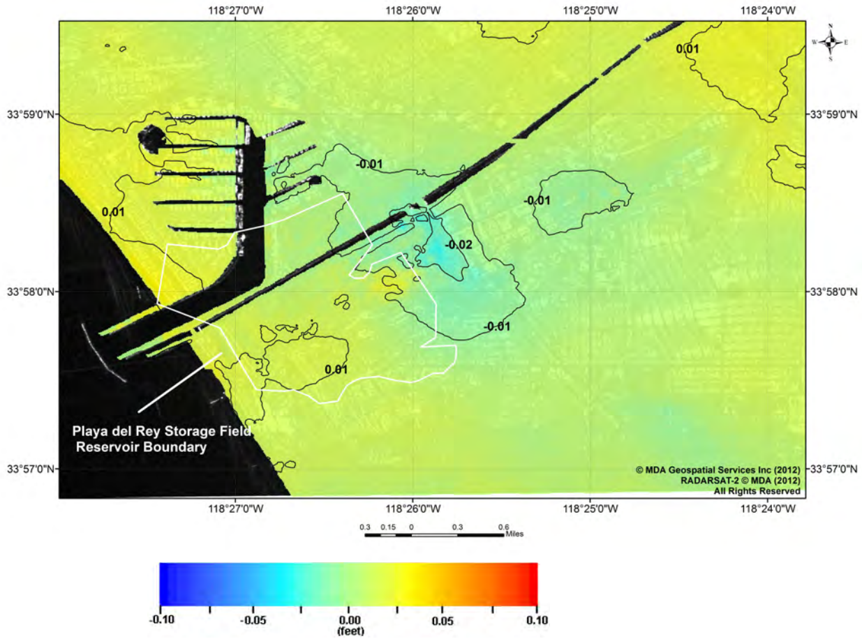
Figure 4: Zoom-in of Playa del Rey Gas Storage Field AOI. Color representation of the vertical deformation product from December 14, 2011 to March 19, 2012 superimposed on SAR image with 0.01 ft contours. In this representation, blue corresponds to subsidence and red would indicate uplift.
