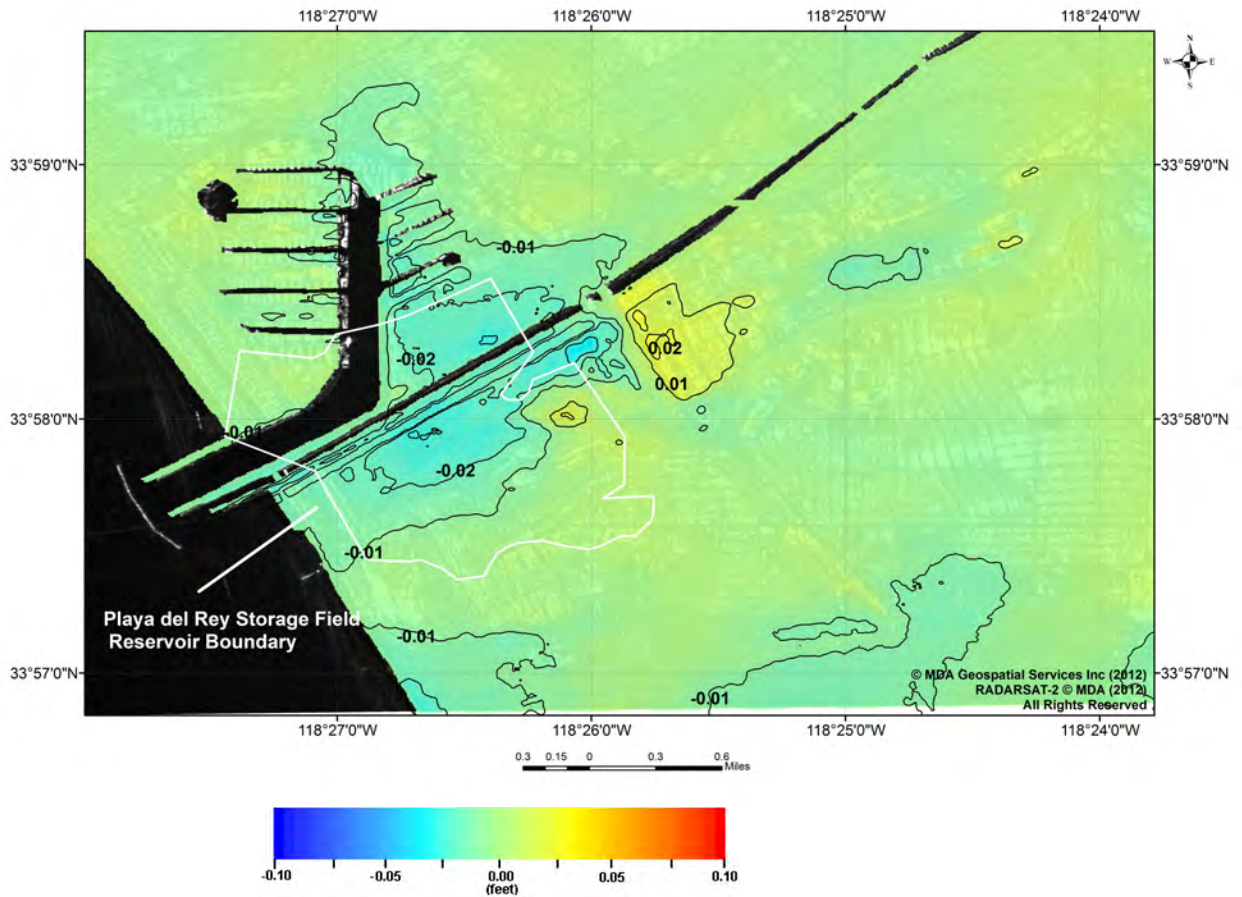
Figure 9: Zoom-in of Playa del Rey Gas Storage Field. Color representation of the summation of the vertical deformation products from December 14, 2011 to June 23, 2012 superimposed on SAR image with 0.01 ft contours. In this representation, blue corresponds to subsidence and red would indicate uplift.
