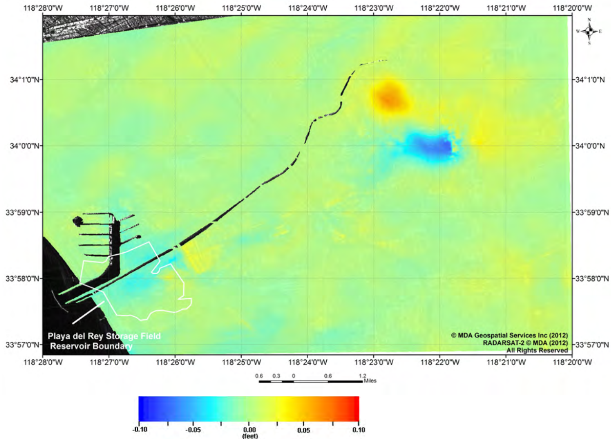
Figure 8: Zoom-in of Playa del Rey Gas Storage Field. Color representation of the summation of the vertical deformation products from December 14, 2011 to June 23, 2012 superimposed on SAR image with 0.01 ft contours. In this representation, blue corresponds to subsidence and red indicates uplift.
