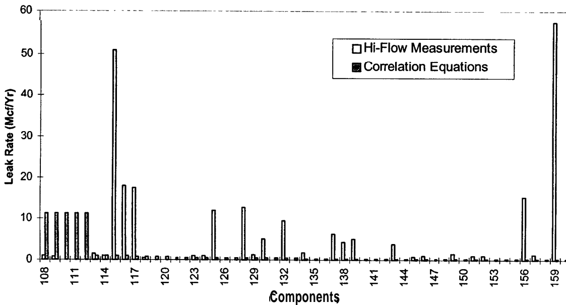
Figure 3. Comparison of Leak Rate Estimates Using Emission Factors and Hi-Flow Measurements - Sorted w.r.t Emission Factor Size
