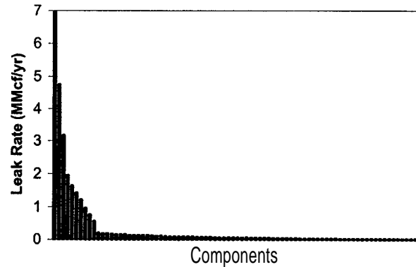
Figure 2. Site 1 - Leak Rate Distribution
