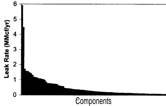
Figure 1. Site 6 - Leak Rate Distribution
