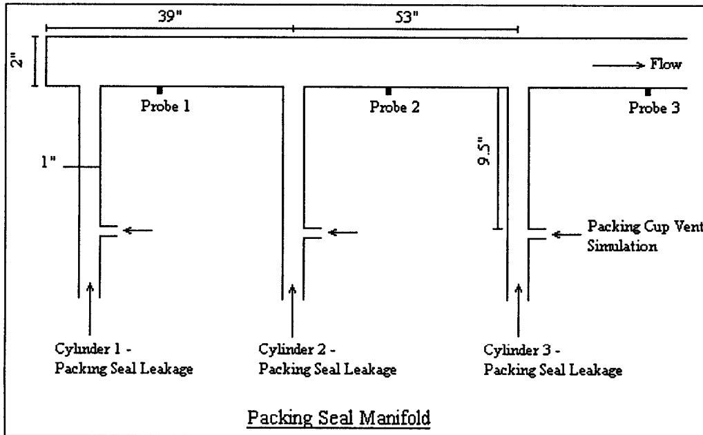
Figure 4. Test Manifold for Monitoring Rod Packing Leakage with Hot Wire Anemometer
