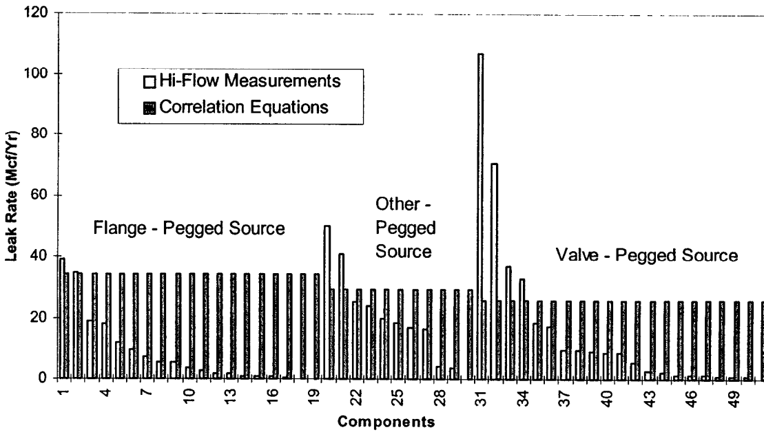
Figure 1. Comparison of Leak Rate Estimates using Correlation Equations and Hi-Flow Measurements -Sorted w.r.t Emission Factor Size
