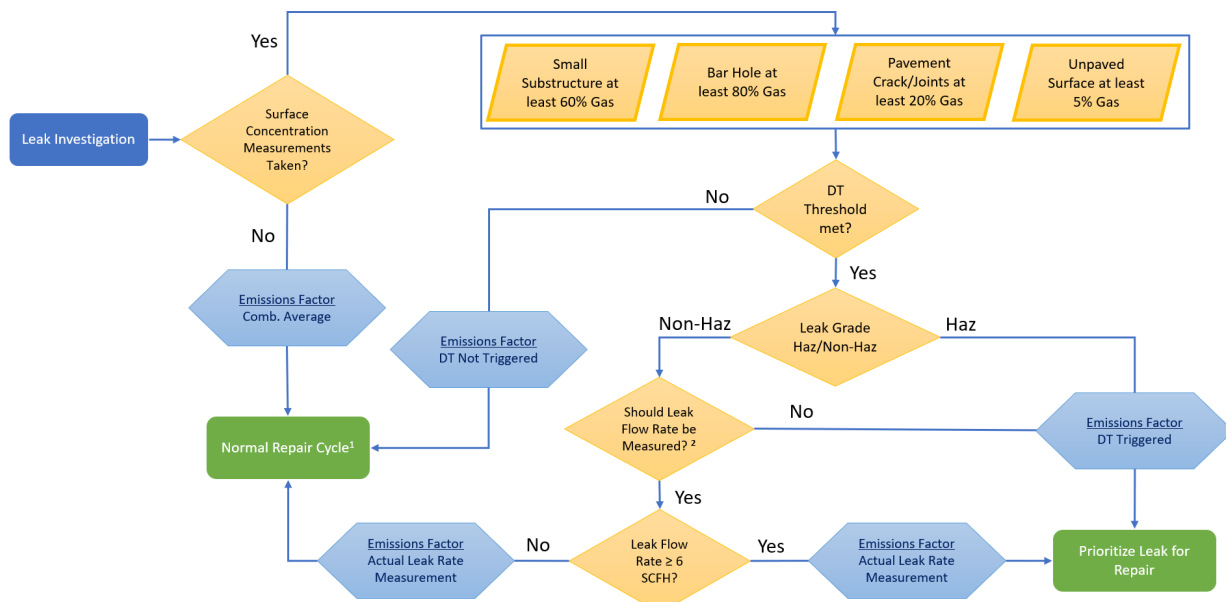
Figure 1. The Leak Investigation Decision Tree
